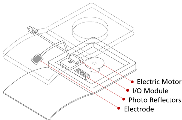
Figure 3: Toolkit overview: electrodes for capacitive sensing, photo reflection sensors, a motor and an I/O module etc.
